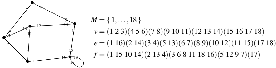
Fig. 1. A planar map represented by permutations
